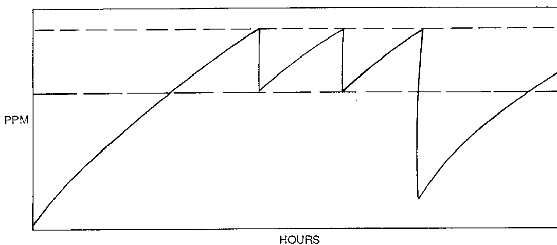
FIGURE 3. Effect of Periodic Fluid Addition and Fluid Change
