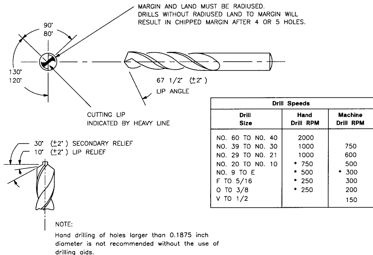
Figure 8-19. Drills for Titanium
