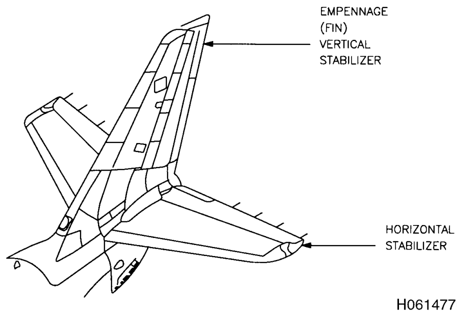
Figure 1-4. Typical Tail Structures
